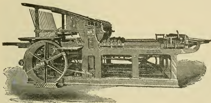
LITHOGRAPHIC PRESS.
